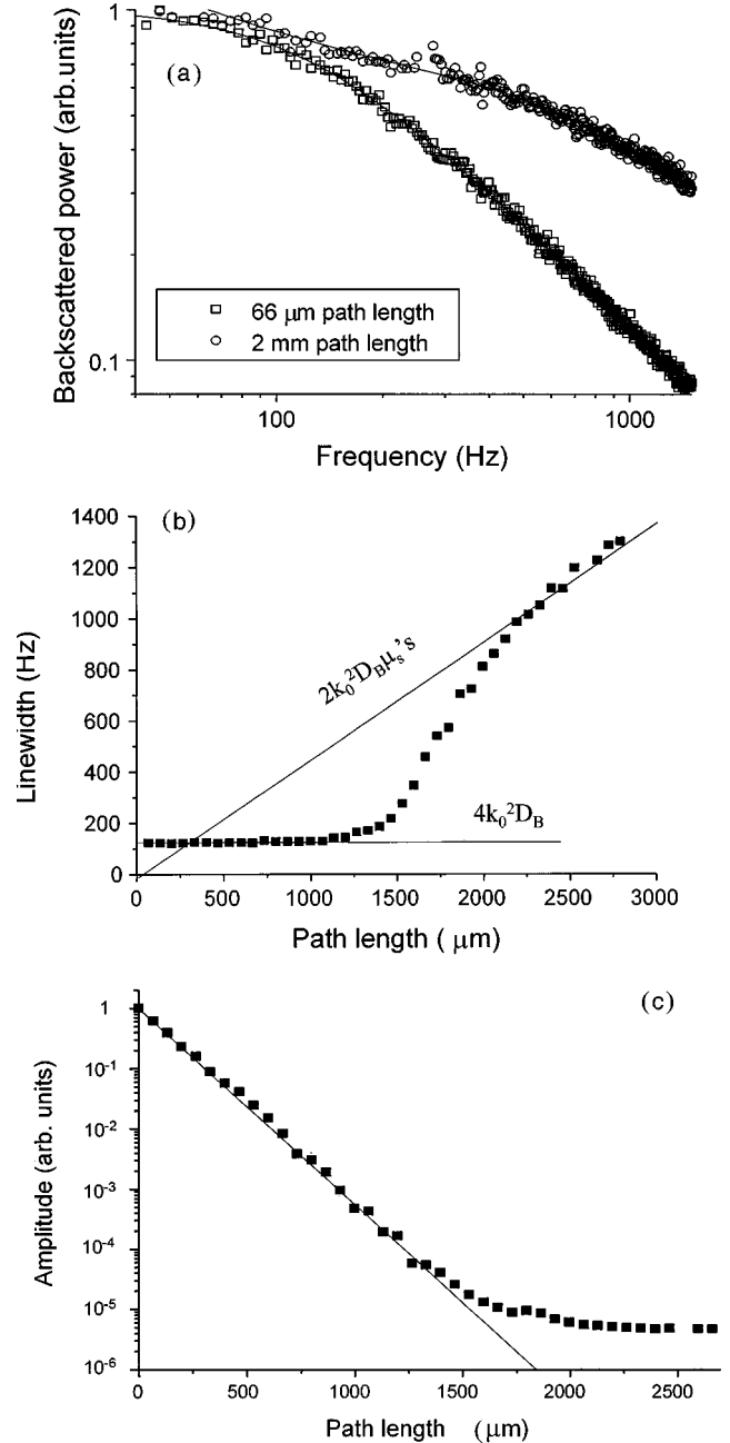
FIG. 2. (a) Power spectrum measured at depths of 66 \mu\text{m} and 2 mm below the sample surface. The solid curves indicate the Lorentzian fits. (b) Lorentzian linewidth as a function of the path length through the scattering medium. The solid lines indicate the expected linewidth behavior in the single scattering and light diffusion regimes, respectively. (c) Lorentzian amplitude as a function of the path length through the scattering medium. The solid line indicates the expected exponential decay in the single scattering regime.
